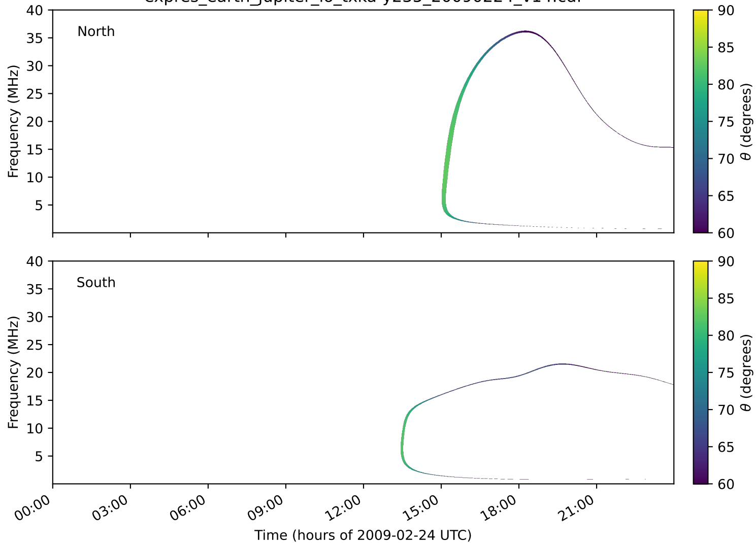
expres_earth_jupiter_io_txka-y235_20090224_v14.cdf
