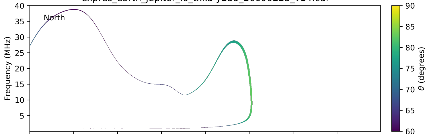
expres_earth_jupiter_io_txka-y235_20090223_v14.cdf
