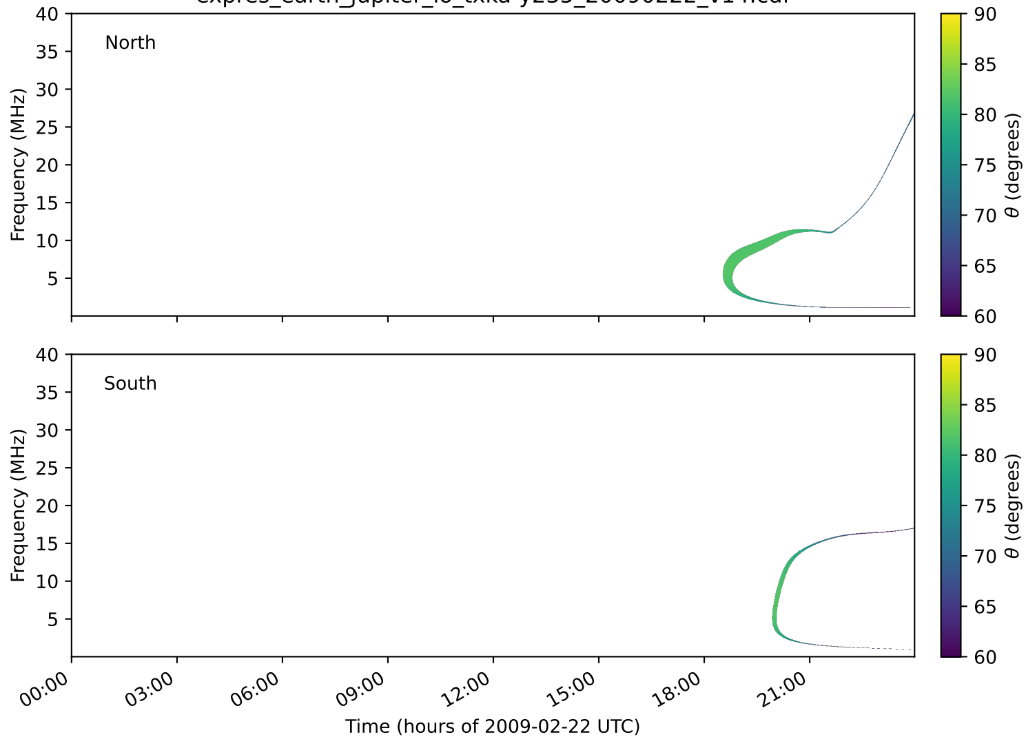
expres_earth_jupiter_io_txka-y235_20090222_v14.cdf
