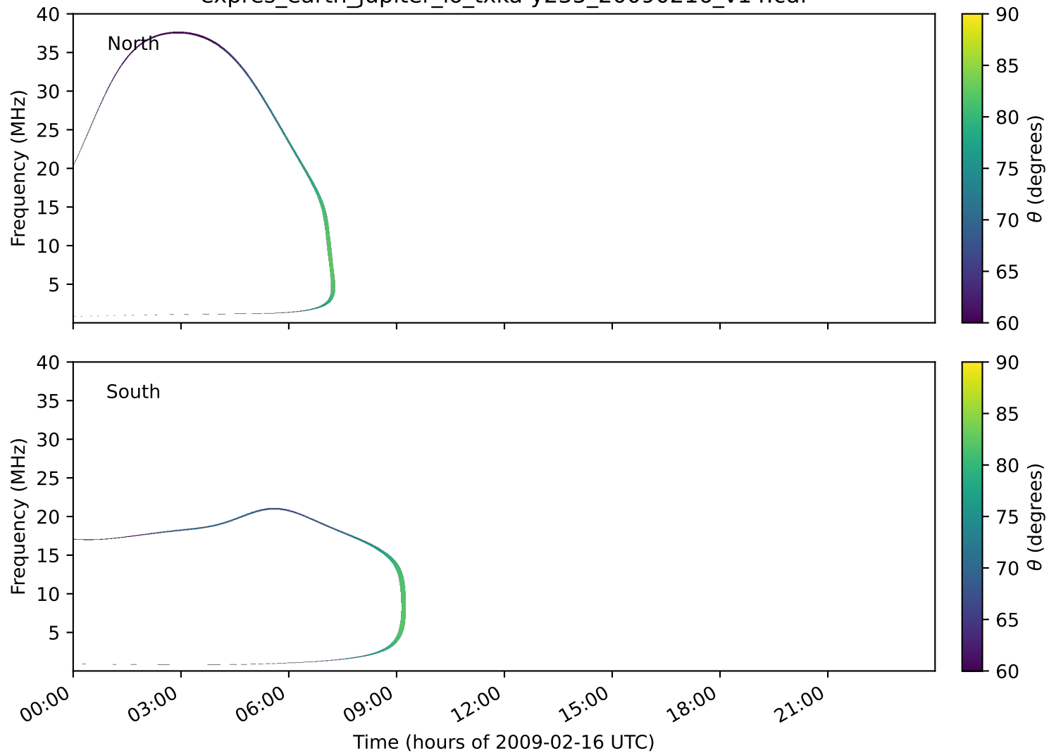
expres_earth_jupiter_io_txka-y235_20090216_v14.cdf
