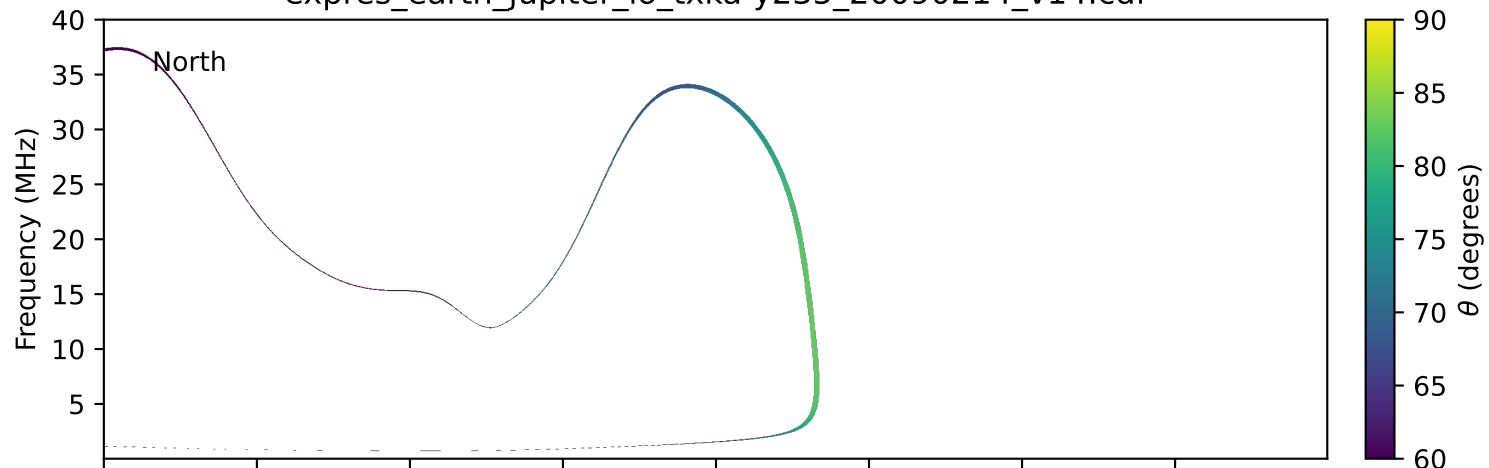
expres_earth_jupiter_io_txka-y235_20090214_v14.cdf
