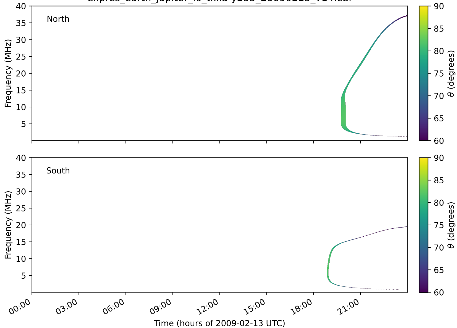
expres_earth_jupiter_io_txka-y235_20090213_v14.cdf
