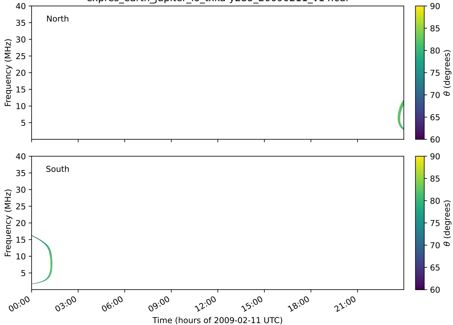
expres_earth_jupiter_io_txka-y235_20090211_v14.cdf
