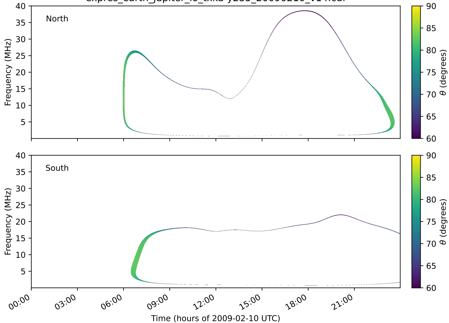
expres_earth_jupiter_io_txka-y235_20090210_v14.cdf
