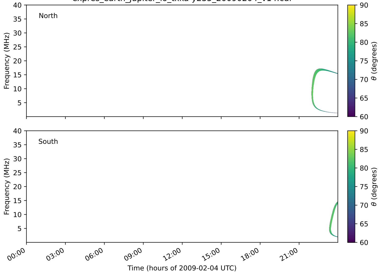
expres_earth_jupiter_io_txka-y235_20090204_v14.cdf
