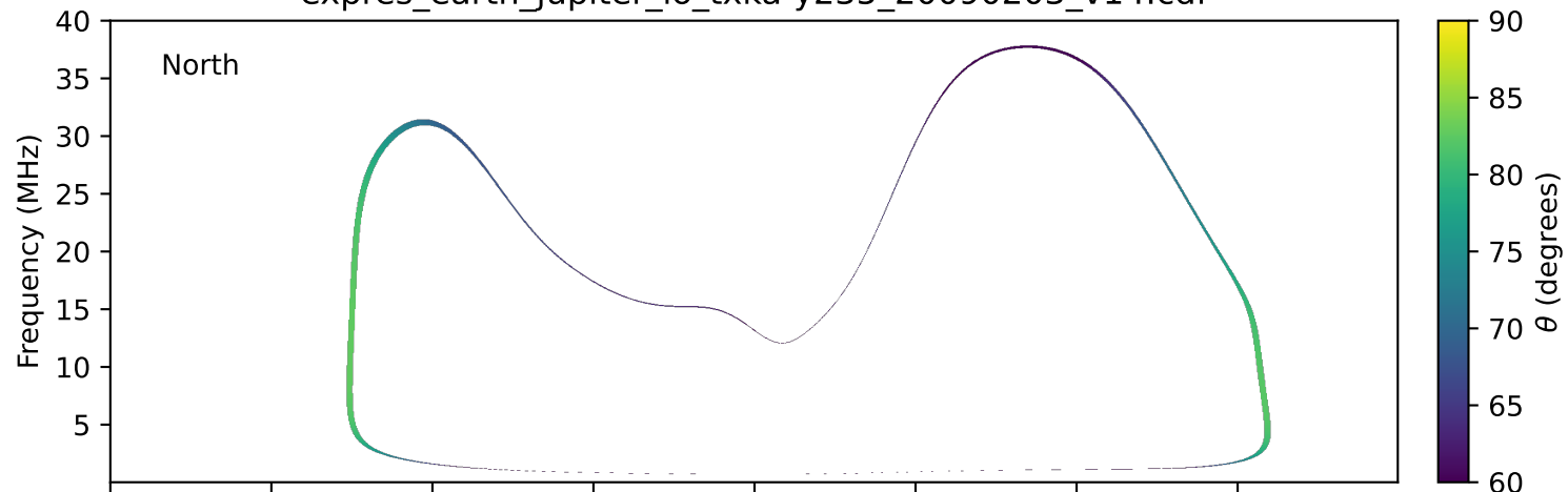
expres_earth_jupiter_io_txka-y235_20090203_v14.cdf
