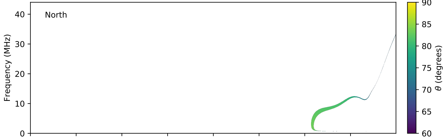
expres_earth_jupiter_io_jrm09_lossc-wid1deg_3kev_20090222_v01.cdf
