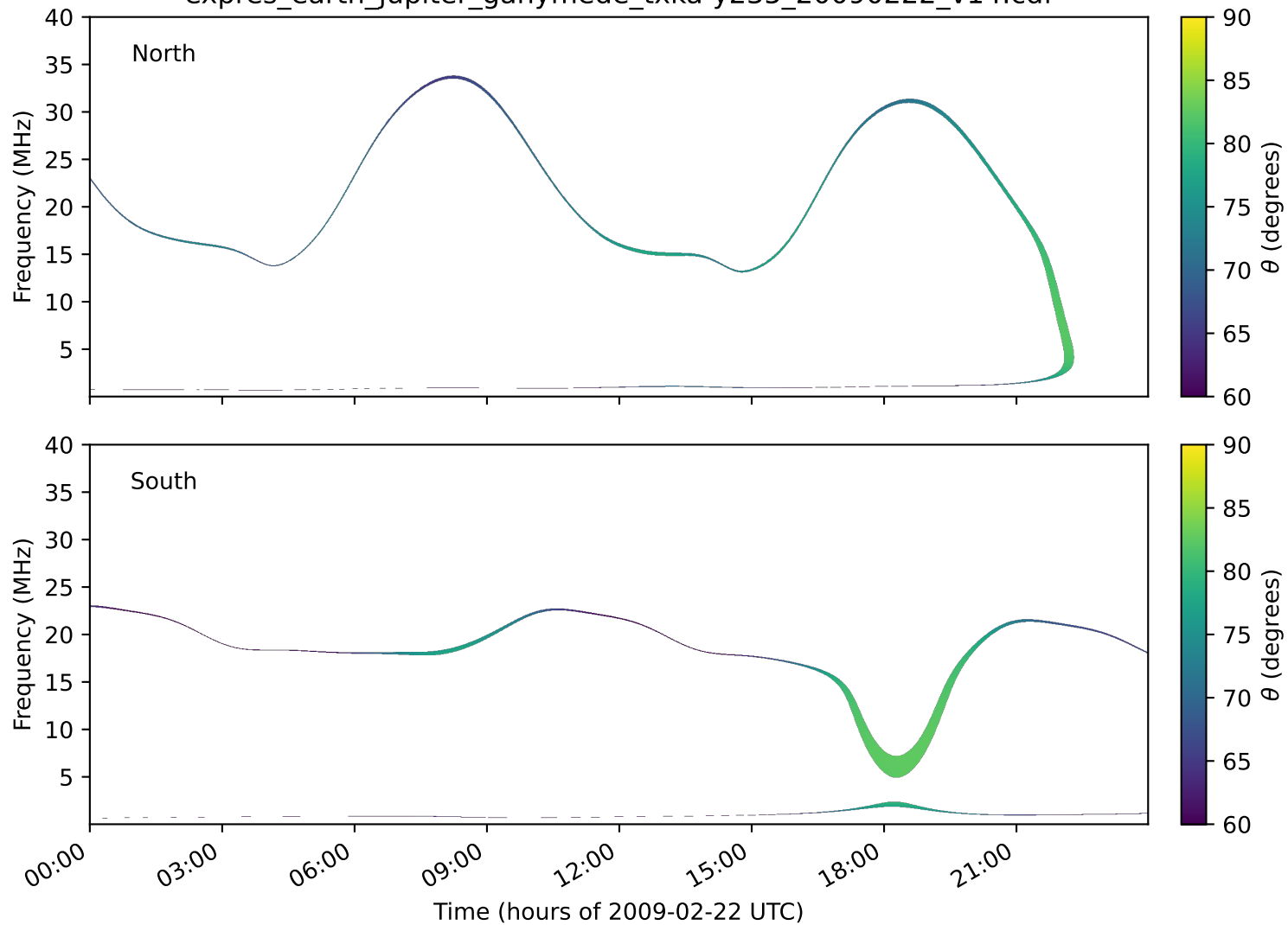
expres_earth_jupiter_ganymede_txka-y235_20090222_v14.cdf
