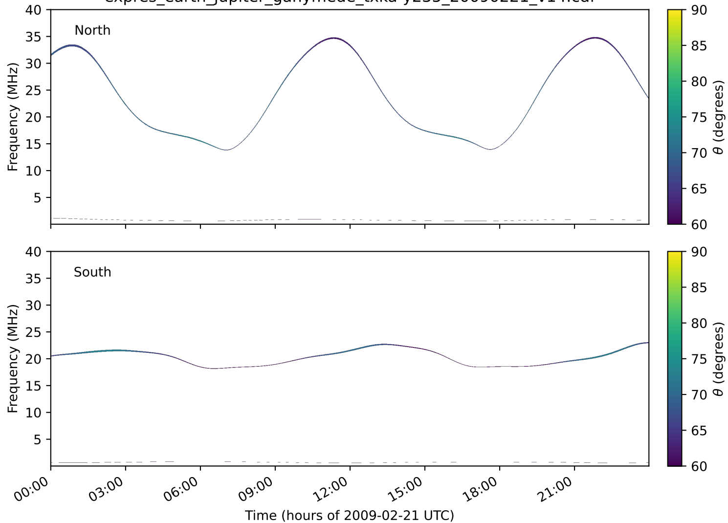
expres_earth_jupiter_ganymede_txka-y235_20090221_v14.cdf
