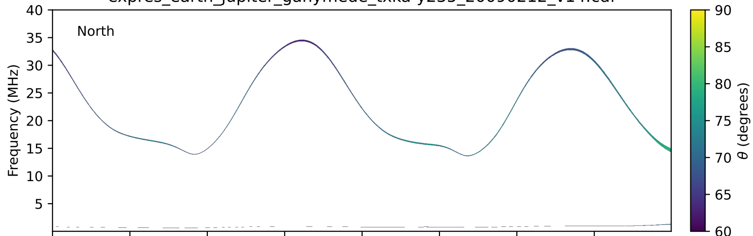
expres_earth_jupiter_ganymede_txka-y235_20090212_v14.cdf
