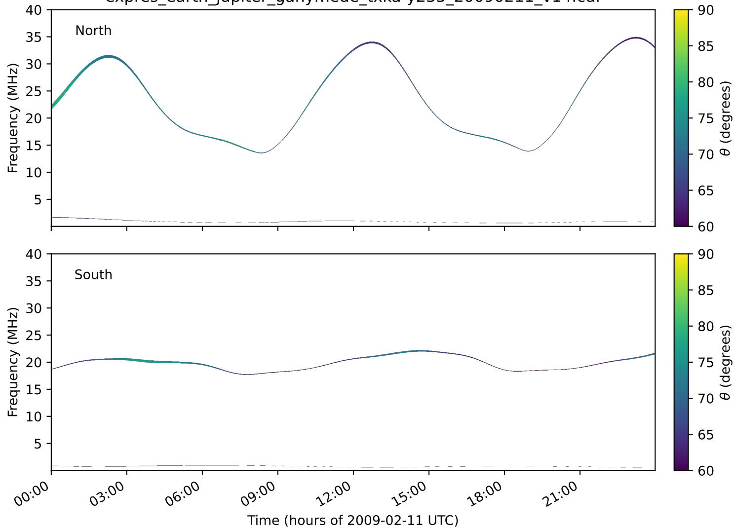
expres_earth_jupiter_ganymede_txka-y235_20090211_v14.cdf
