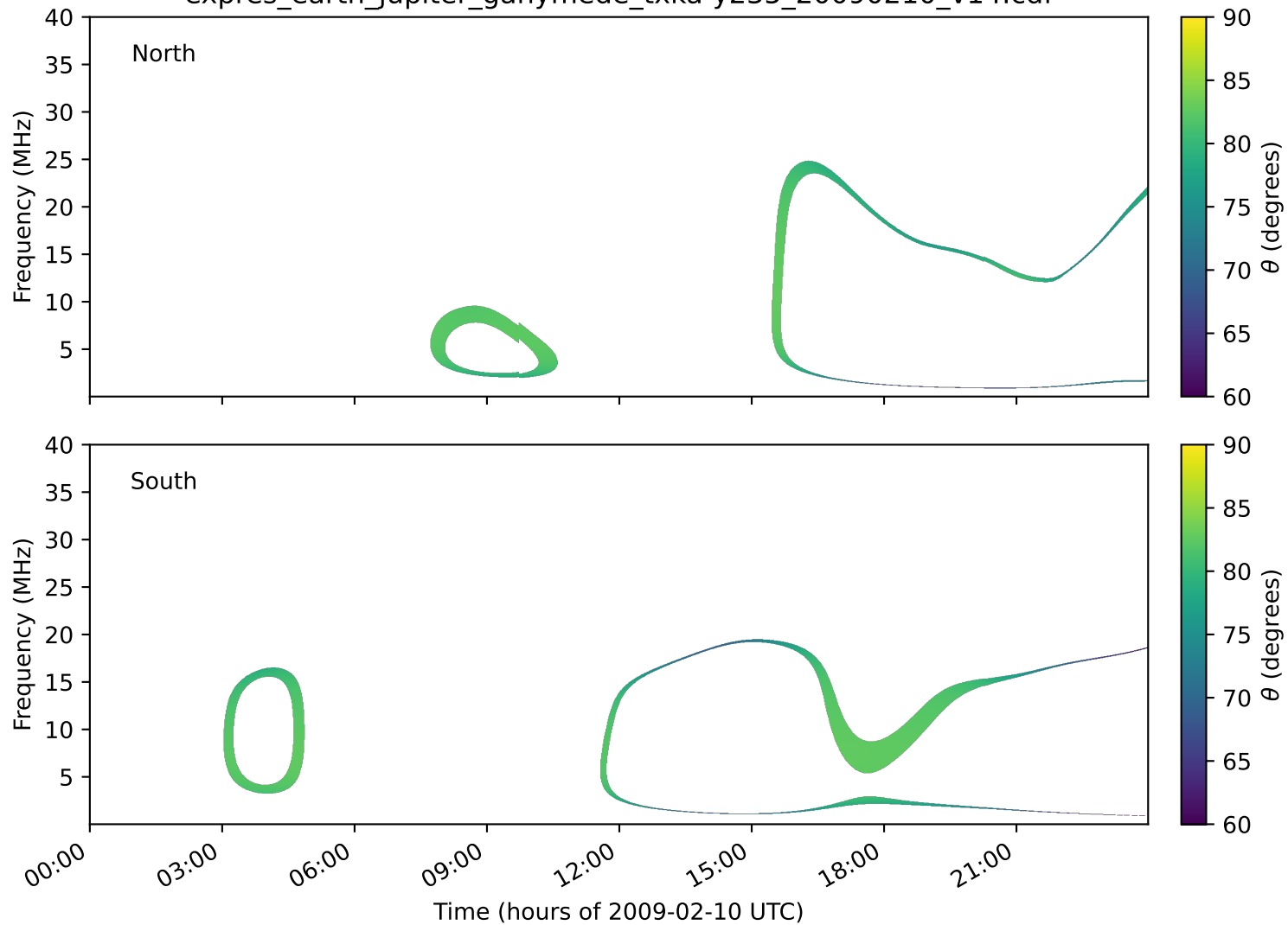
expres_earth_jupiter_ganymede_txka-y235_20090210_v14.cdf
