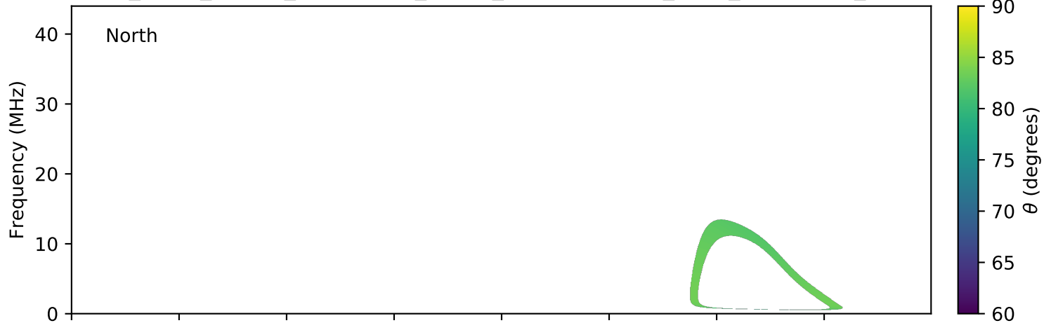
expres_earth_jupiter_ganymede_jrm09_lossc-wid1deg_3kev_20090217_v01.cdf
