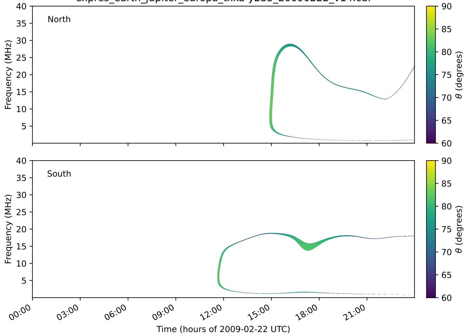
expres_earth_jupiter_europa_txka-y235_20090222_v14.cdf
