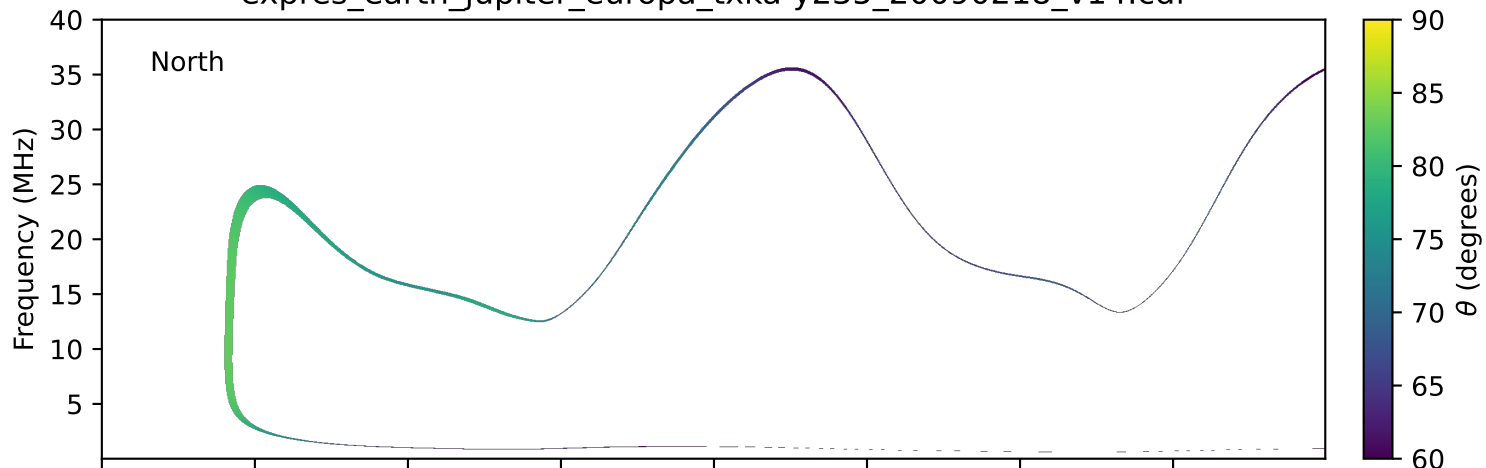
expres_earth_jupiter_europa_txka-y235_20090218_v14.cdf
