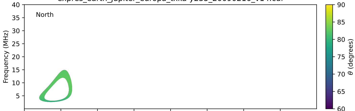
expres_earth_jupiter_europa_txka-y235_20090216_v14.cdf
