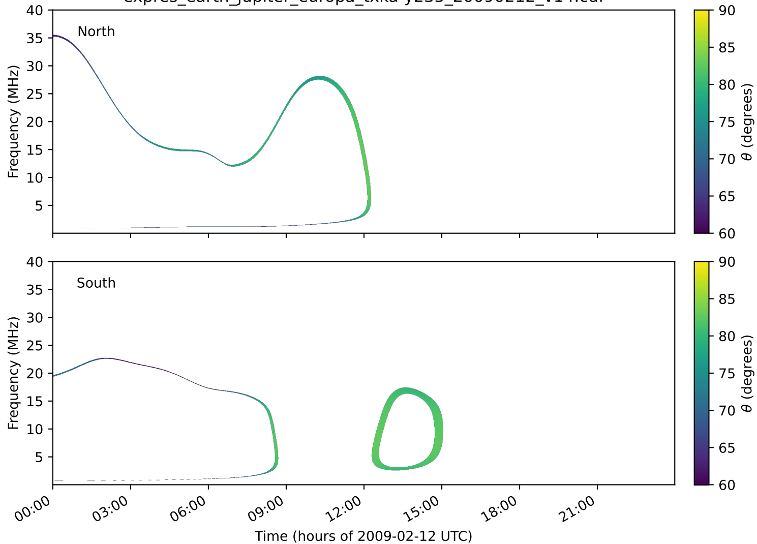
expres_earth_jupiter_europa_txka-y235_20090212_v14.cdf
