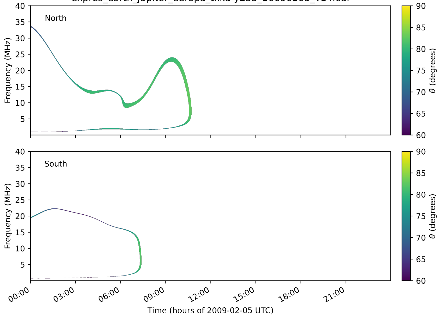
expres_earth_jupiter_europa_txka-y235_20090205_v14.cdf
