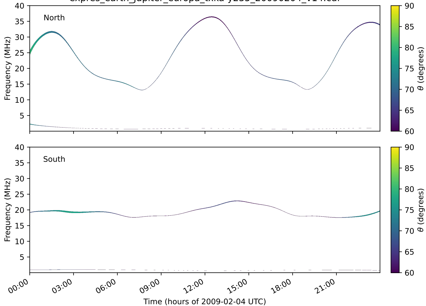
expres_earth_jupiter_europa_txka-y235_20090204_v14.cdf
