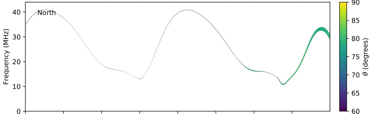
expres_earth_jupiter_europa_jrm09_lossc-wid1deg_3kev_20090216_v01.cdf
