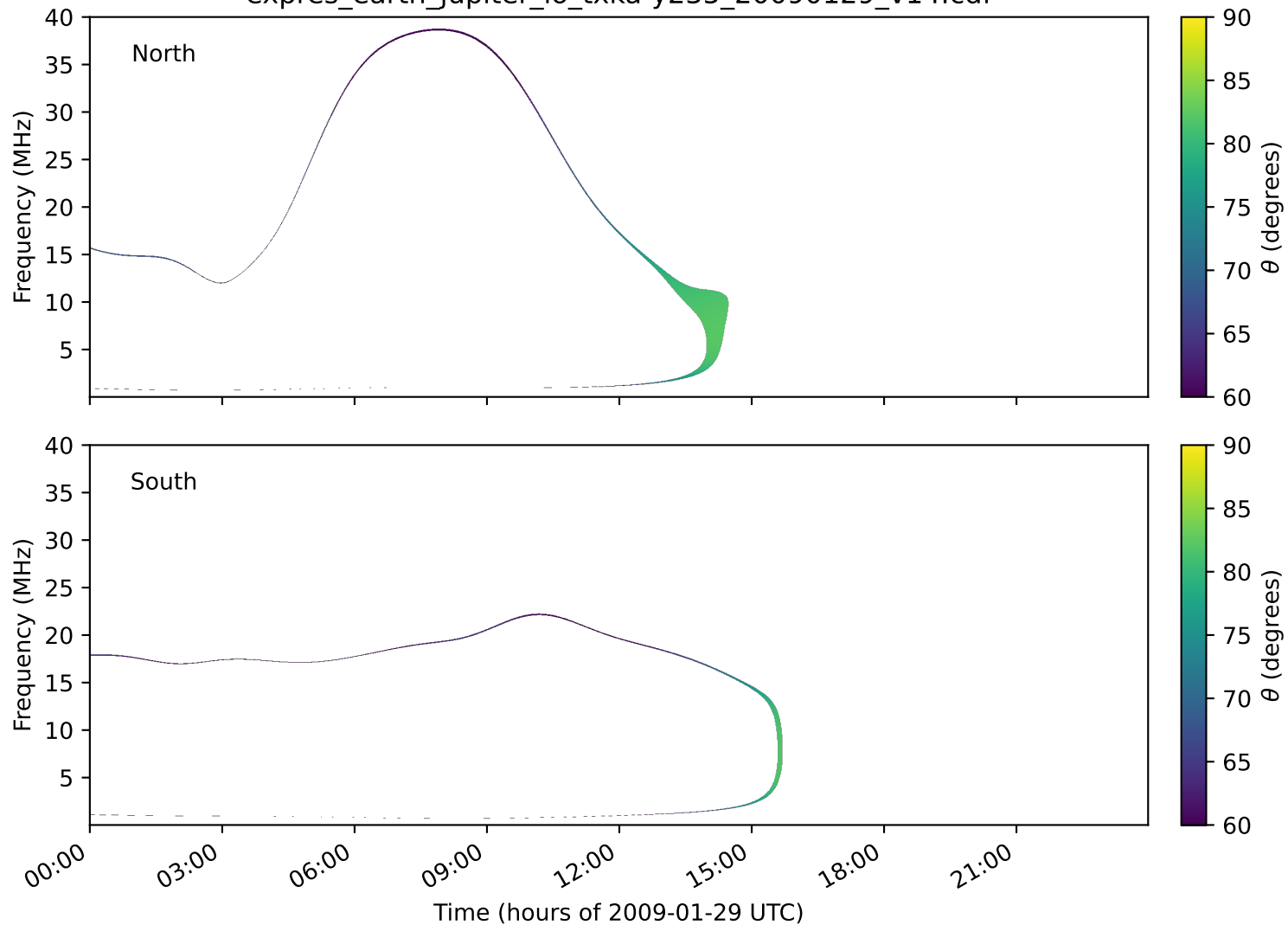
expres_earth_jupiter_io_txka-y235_20090129_v14.cdf
