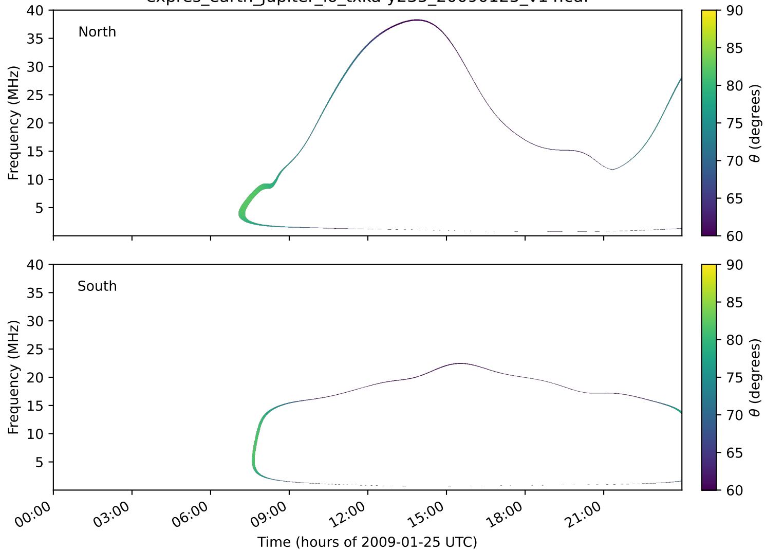
expres_earth_jupiter_io_txka-y235_20090125_v14.cdf
