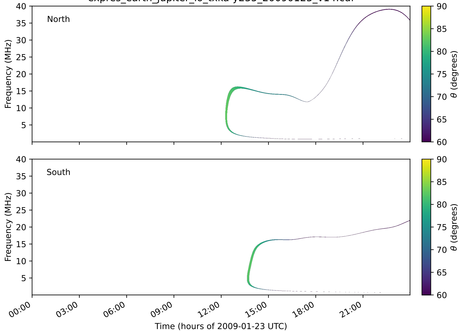
expres_earth_jupiter_io_txka-y235_20090123_v14.cdf
