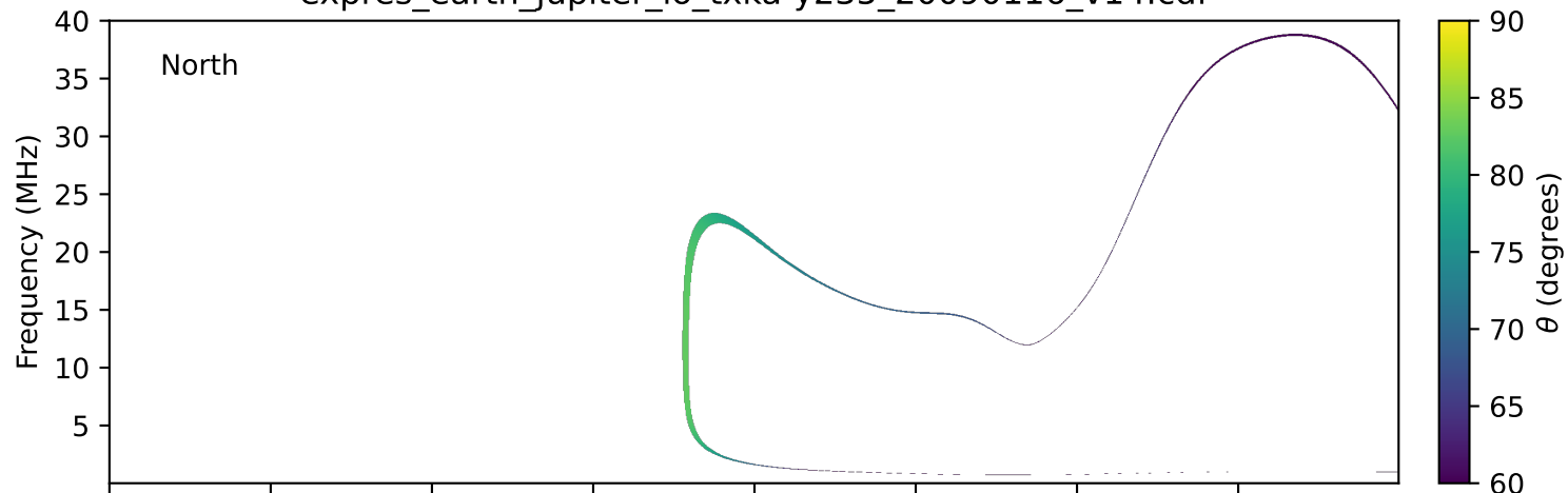
expres_earth_jupiter_io_txka-y235_20090116_v14.cdf
