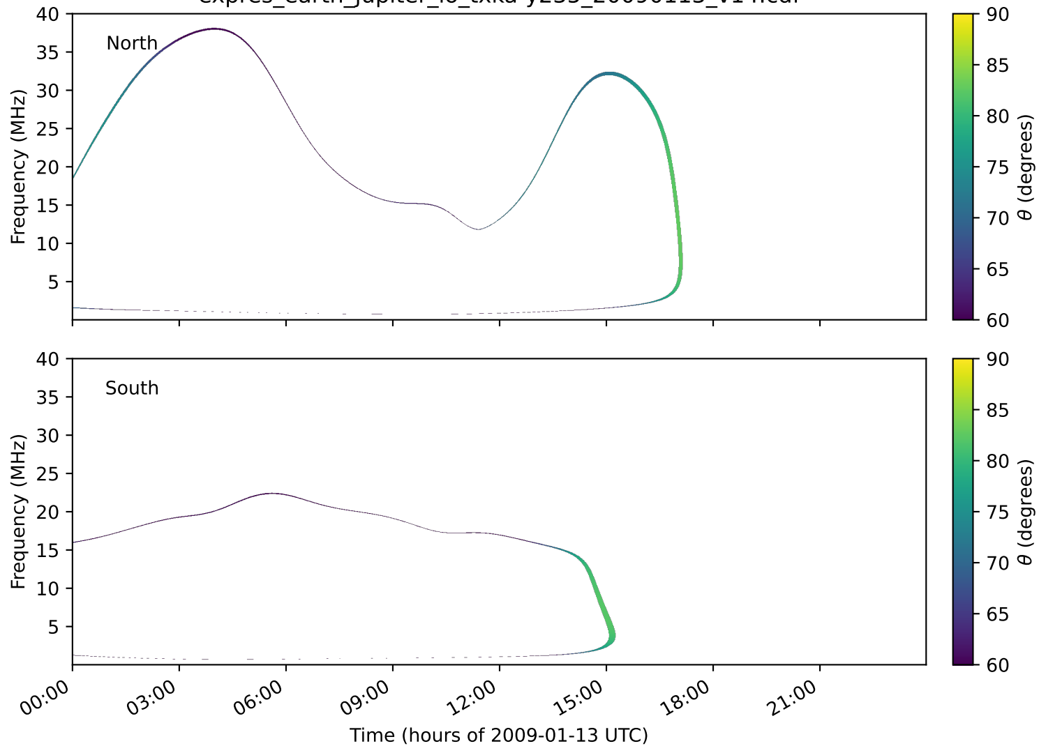
expres_earth_jupiter_io_txka-y235_20090113_v14.cdf
