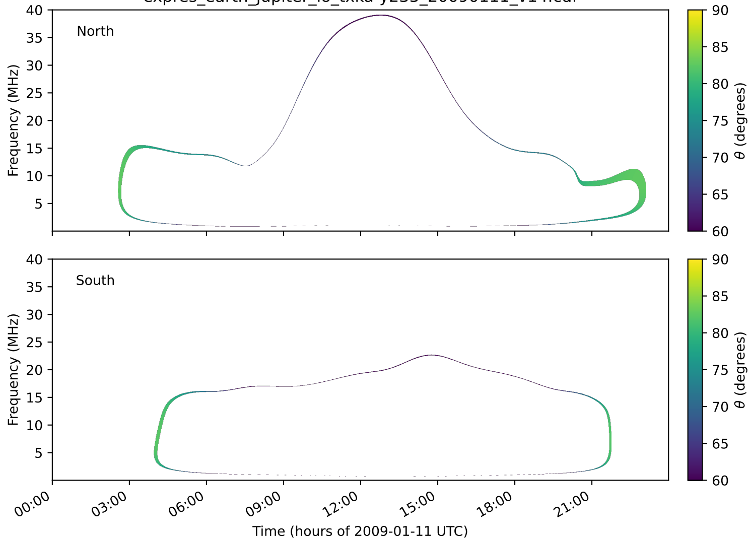
expres_earth_jupiter_io_txka-y235_20090111_v14.cdf
