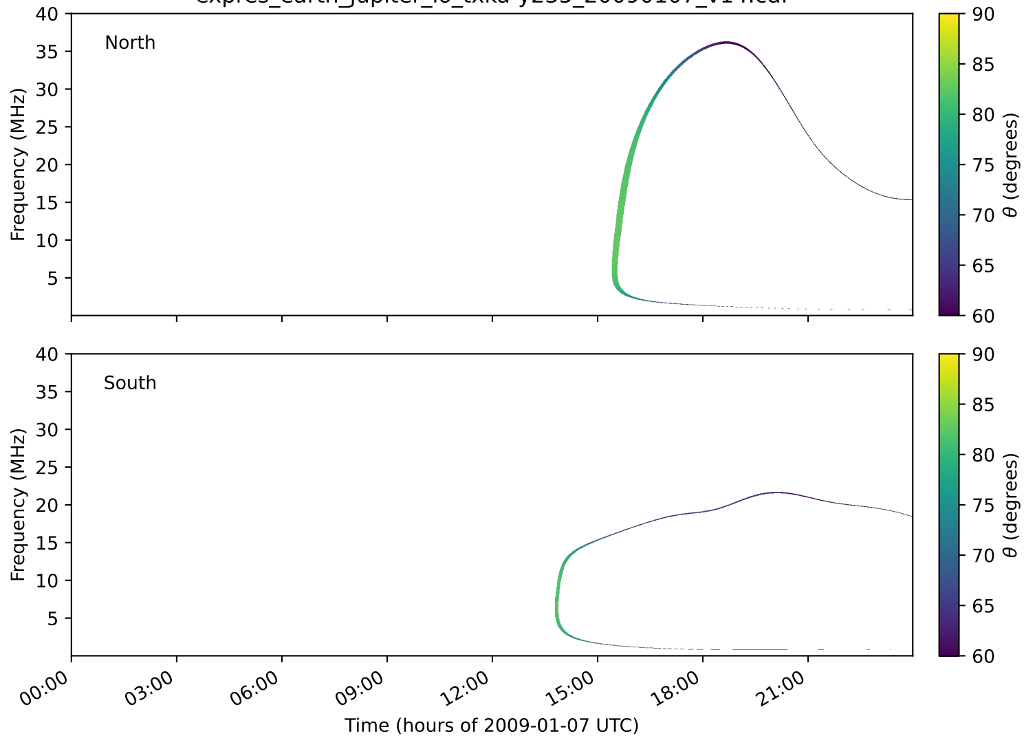
expres_earth_jupiter_io_txka-y235_20090107_v14.cdf
