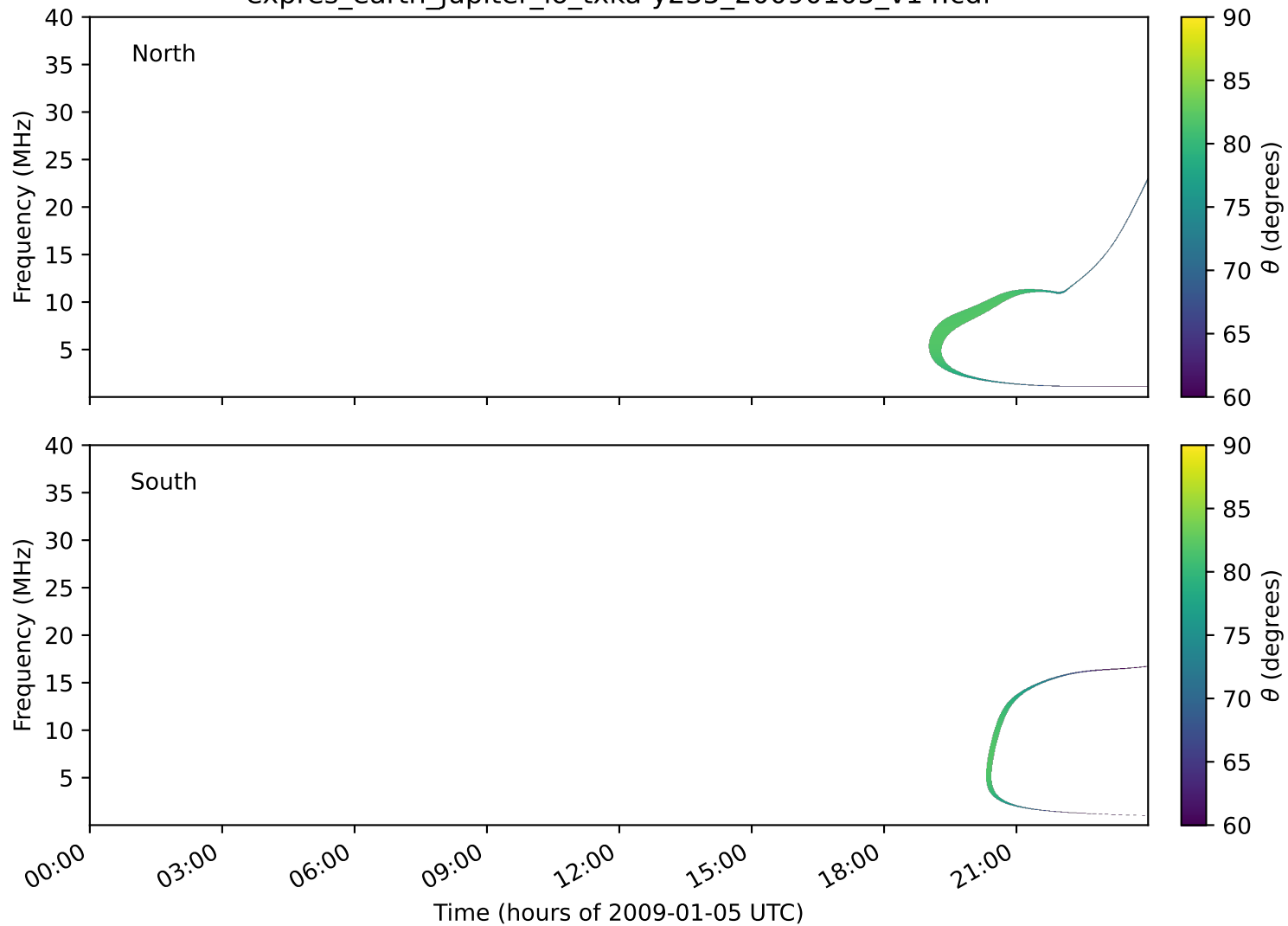
expres_earth_jupiter_io_txka-y235_20090105_v14.cdf
