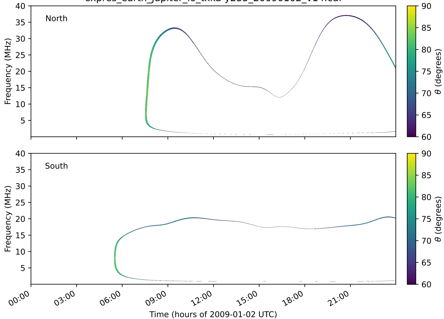
expres_earth_jupiter_io_txka-y235_20090102_v14.cdf
