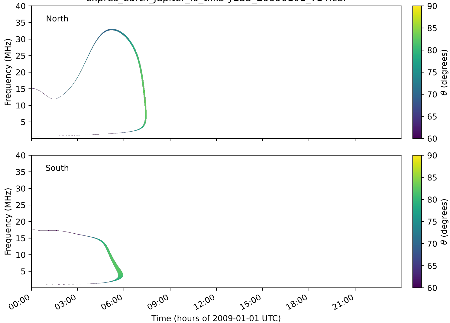
expres_earth_jupiter_io_txka-y235_20090101_v14.cdf
