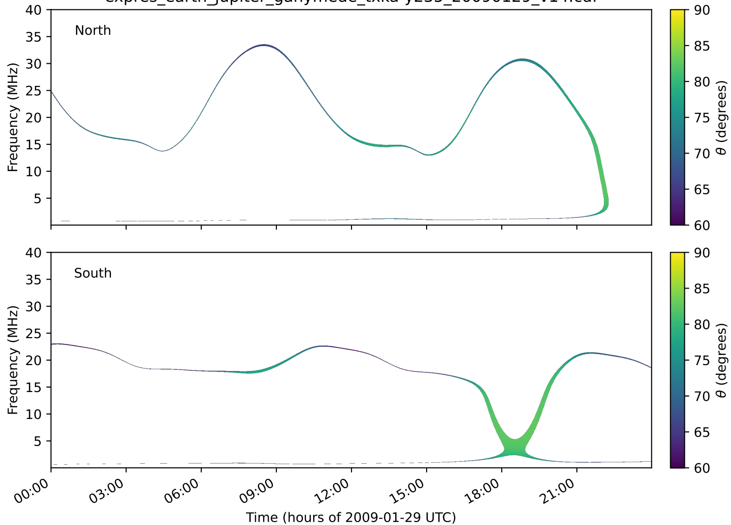
expres_earth_jupiter_ganymede_txka-y235_20090129_v14.cdf
