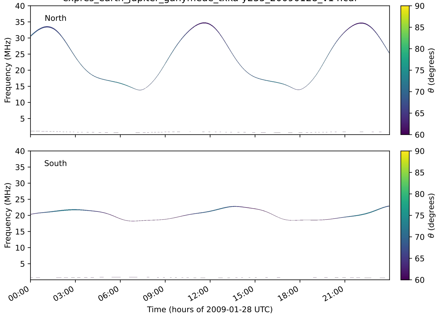
expres_earth_jupiter_ganymede_txka-y235_20090128_v14.cdf
