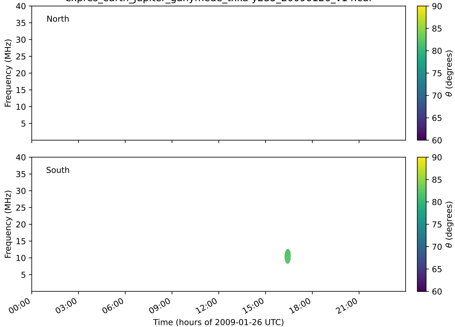
expres_earth_jupiter_ganymede_txka-y235_20090126_v14.cdf
