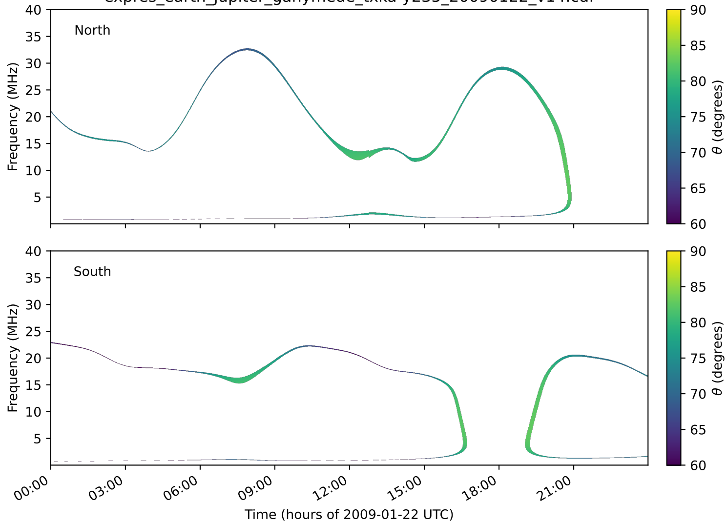
expres_earth_jupiter_ganymede_txka-y235_20090122_v14.cdf
