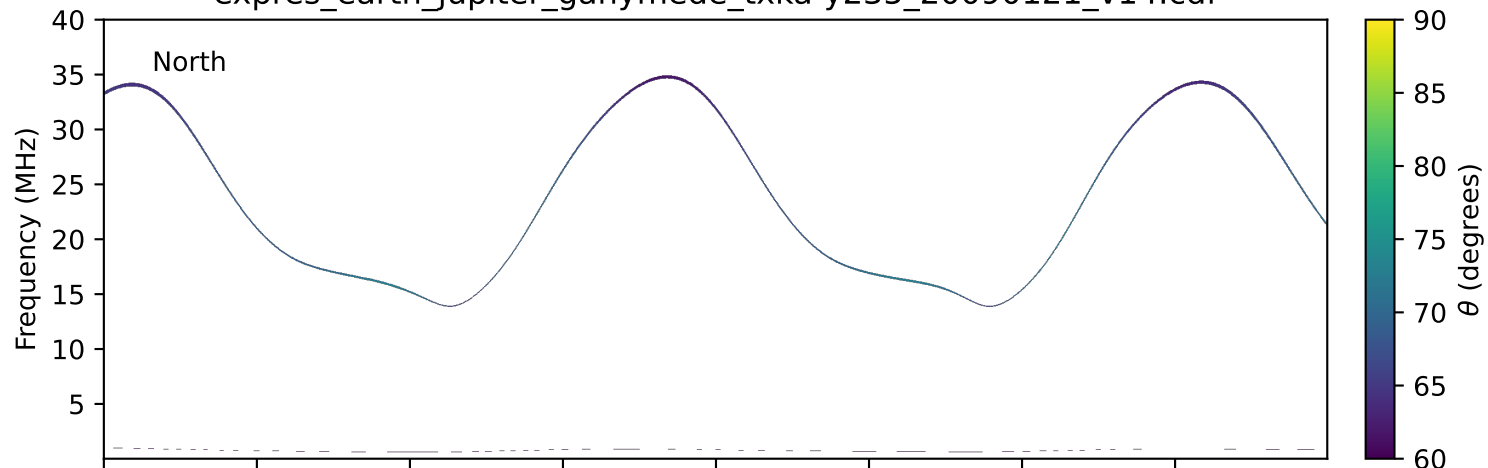
expres_earth_jupiter_ganymede_txka-y235_20090121_v14.cdf
