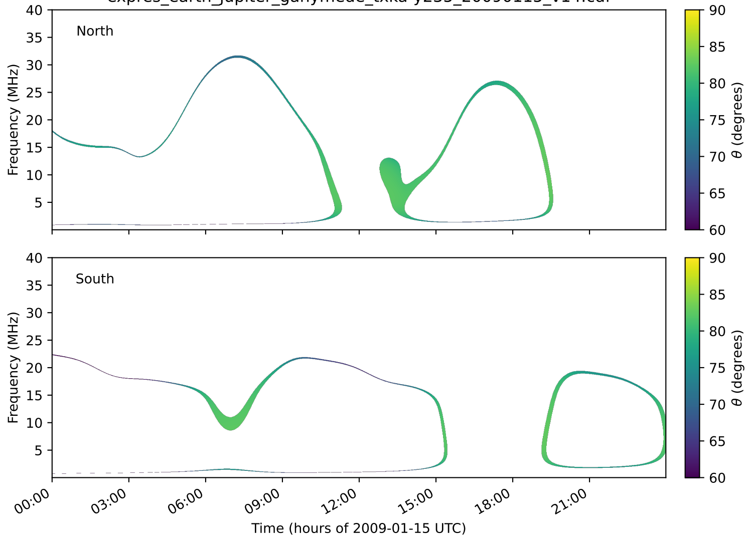
expres_earth_jupiter_ganymede_txka-y235_20090115_v14.cdf
