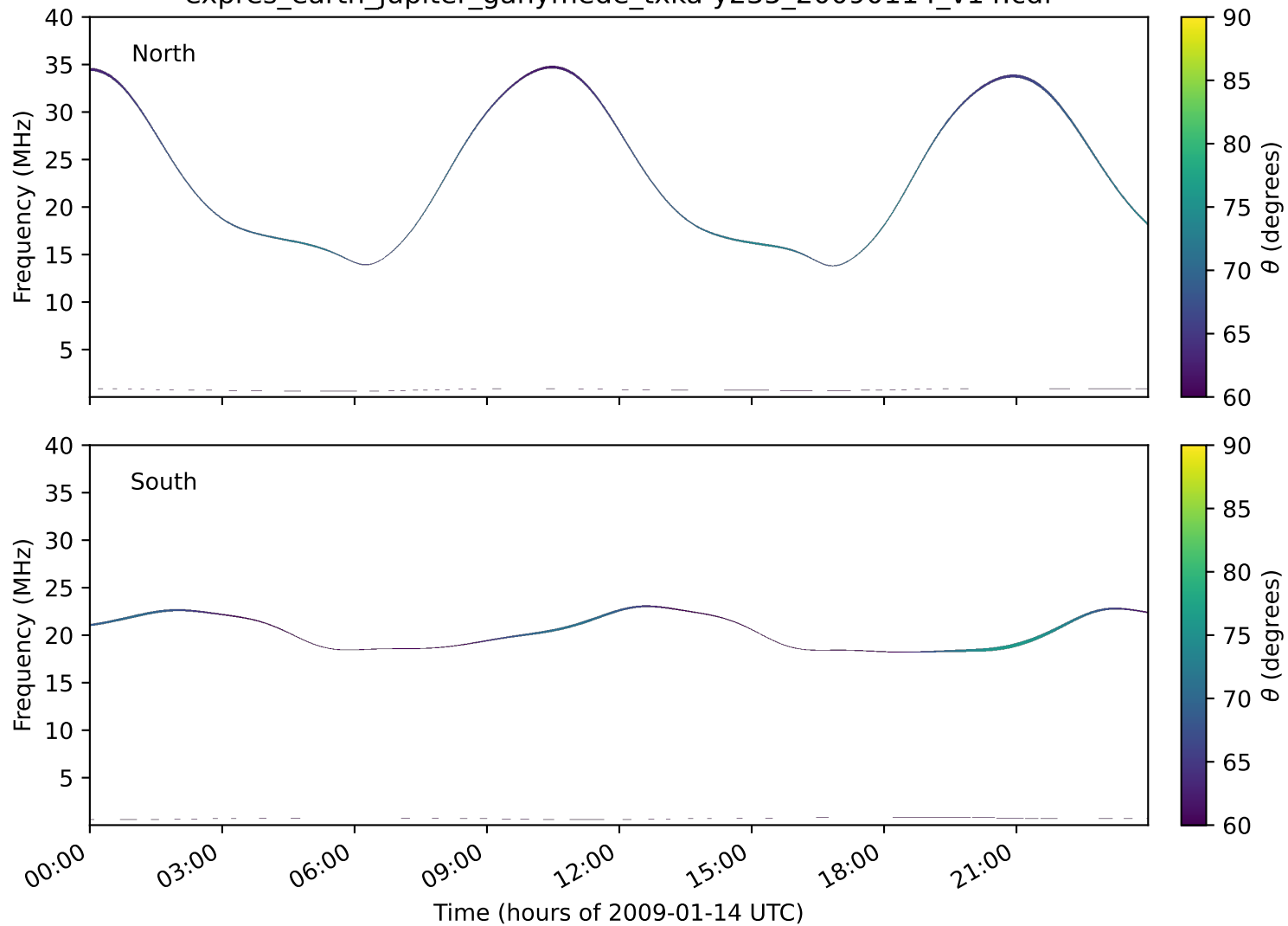
expres_earth_jupiter_ganymede_txka-y235_20090114_v14.cdf
