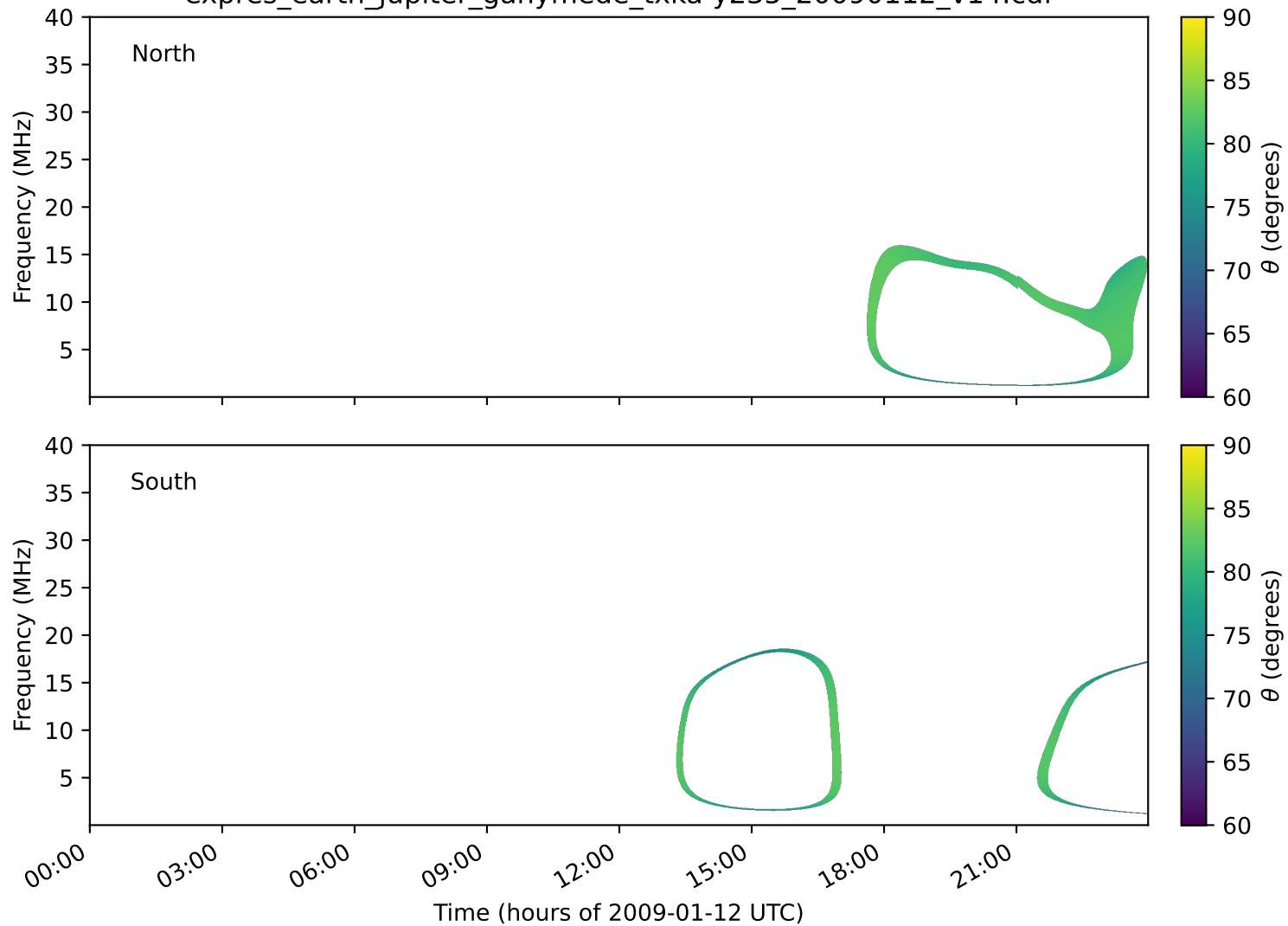
expres_earth_jupiter_ganymede_txka-y235_20090112_v14.cdf
