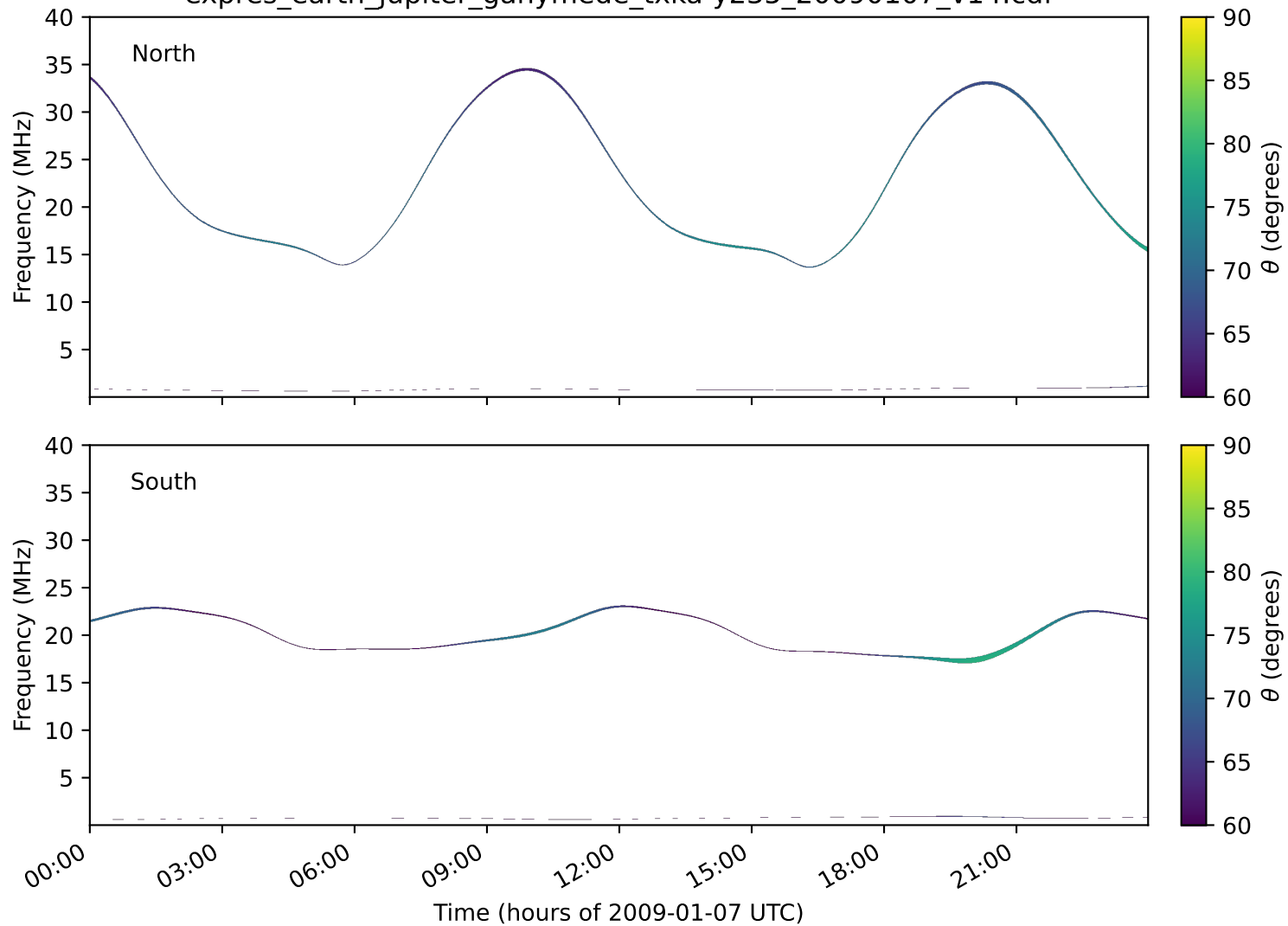
expres_earth_jupiter_ganymede_txka-y235_20090107_v14.cdf
