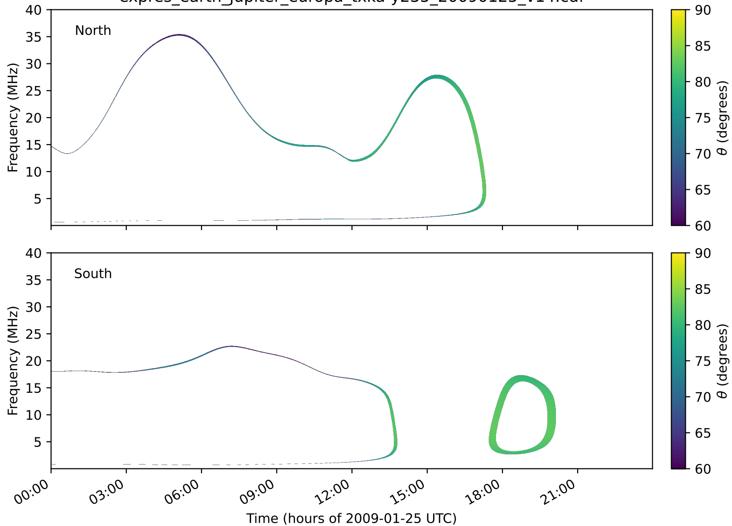
expres_earth_jupiter_europa_txka-y235_20090125_v14.cdf
