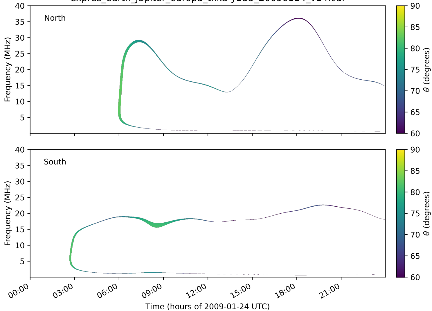
expres_earth_jupiter_europa_txka-y235_20090124_v14.cdf
