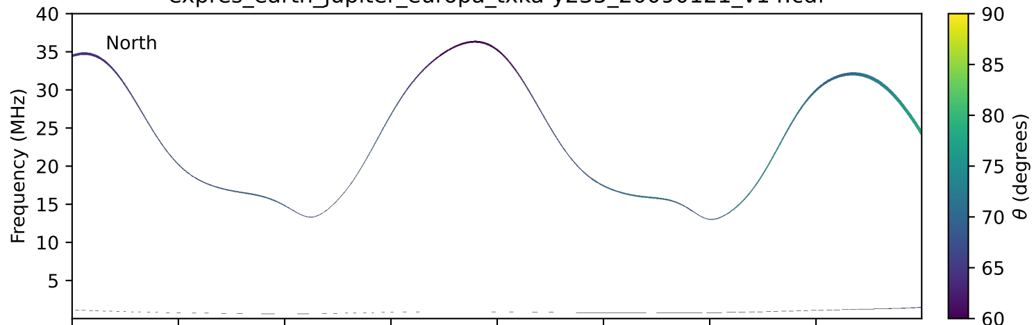
expres_earth_jupiter_europa_txka-y235_20090121_v14.cdf
