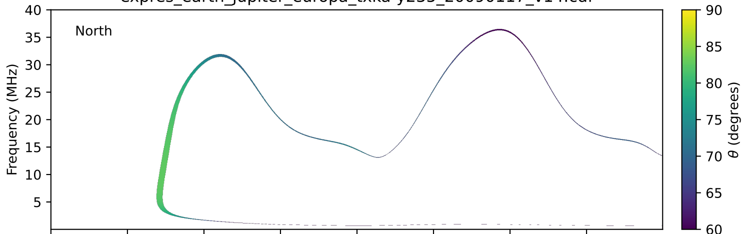
expres_earth_jupiter_europa_txka-y235_20090117_v14.cdf
