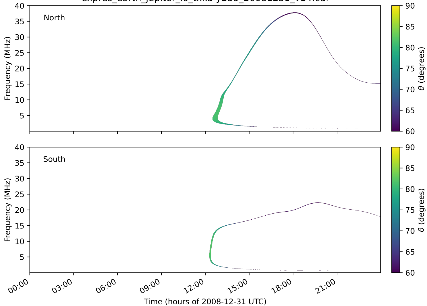
expres_earth_jupiter_io_txka-y235_20081231_v14.cdf
