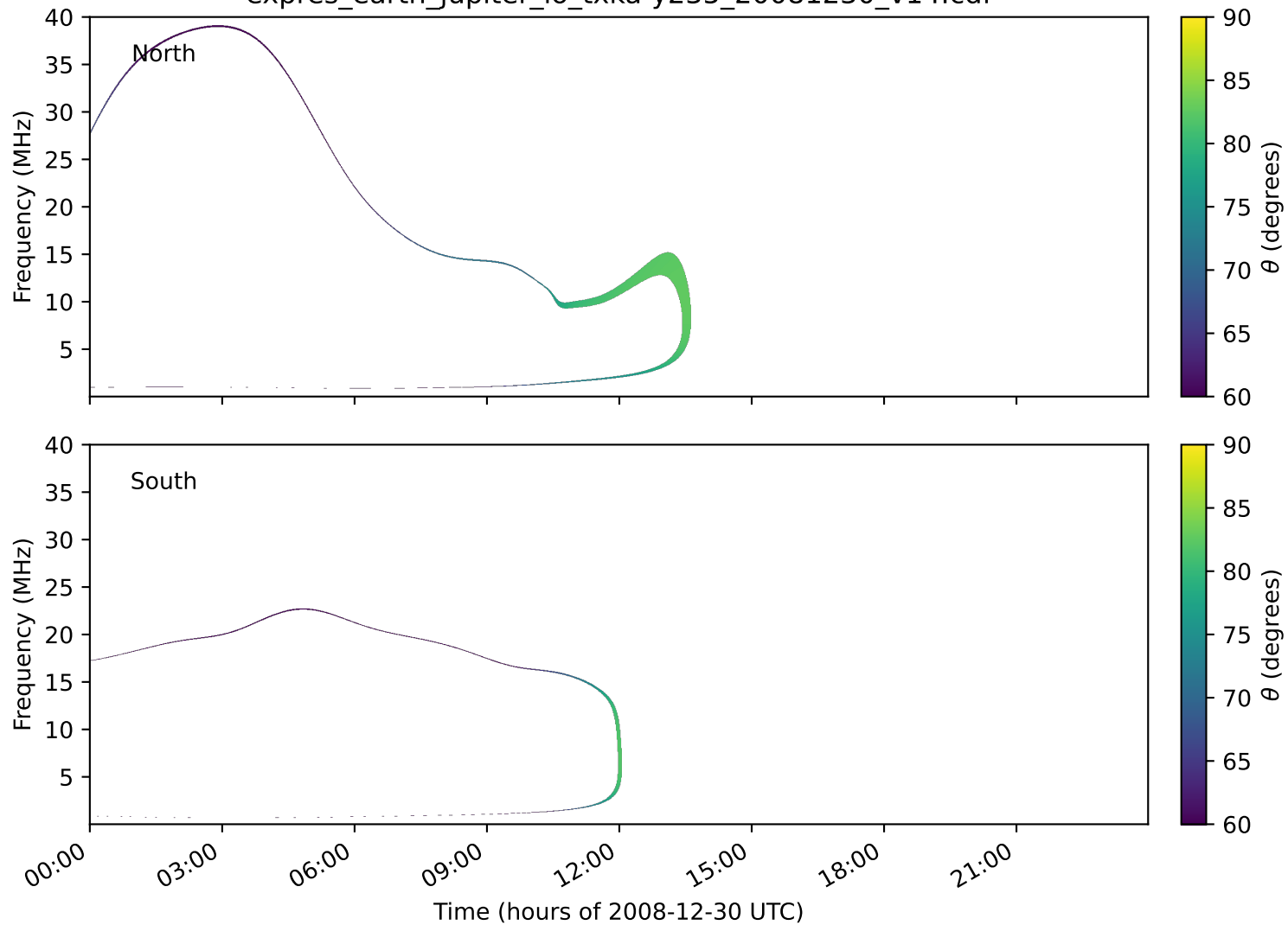
expres_earth_jupiter_io_txka-y235_20081230_v14.cdf
