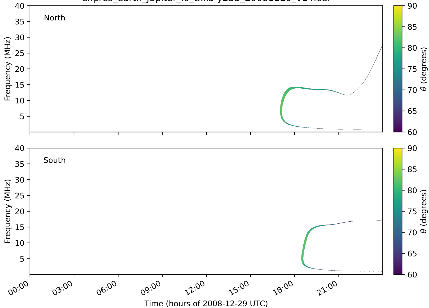
expres_earth_jupiter_io_txka-y235_20081229_v14.cdf
